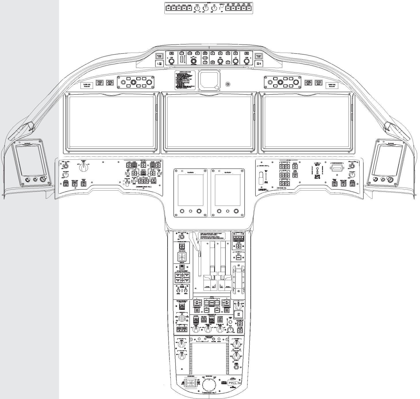
FIGURE III — Citation X+ INSTRUMENT PANEL AND PEDESTAL LAYOUT
